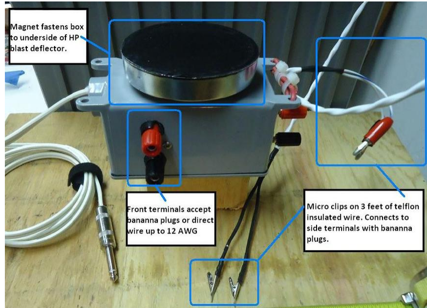
Figure 1 – Grey Terminal Box Front Connections – Direct Wire
