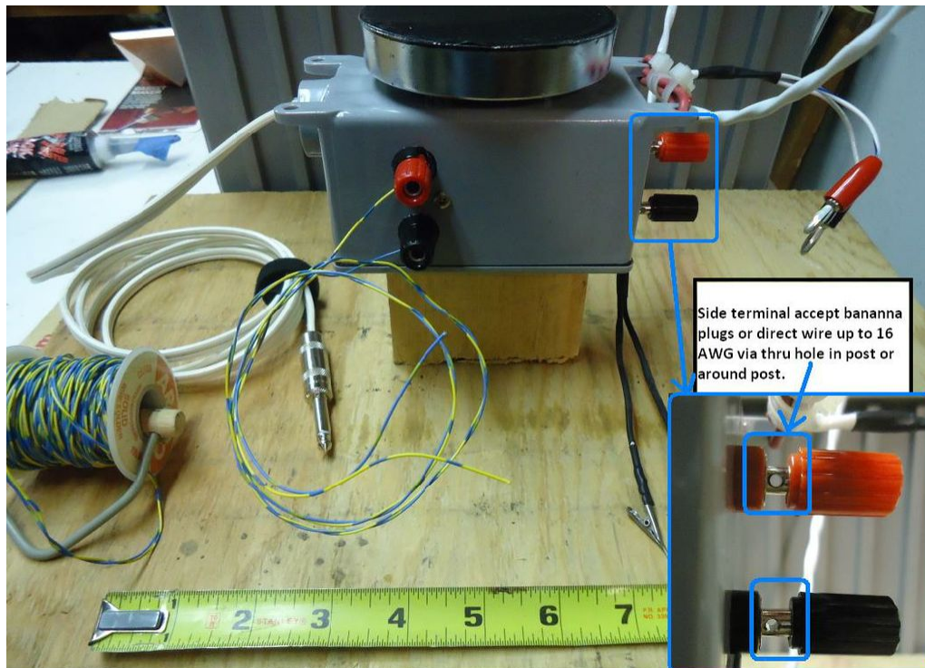
Figure 2 – Grey Terminal Box Side Connections – Direct Wire Or Micro Clips
